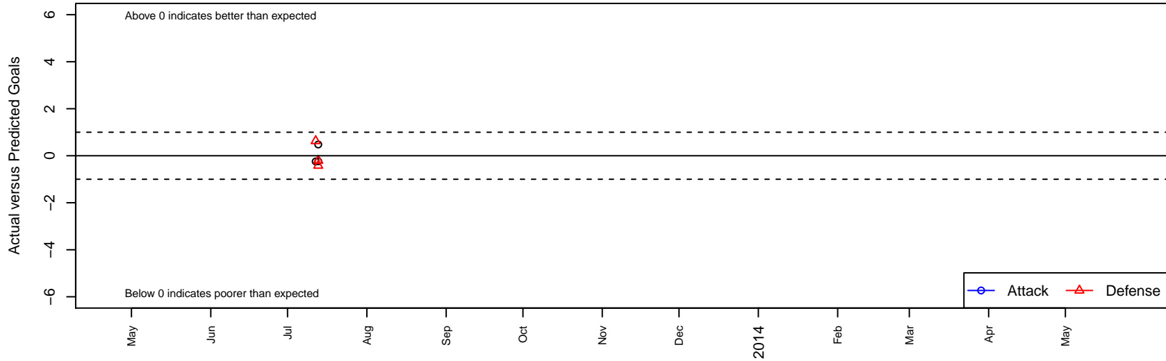
Bellevue Blaze G00 Dots are actual minus expected GF (blue circles) and GA (red triangles). Blue line is smoothed change in attack strength. Red is smoothed change in defense strength.
